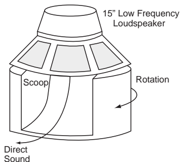
Lower speaker assembly
